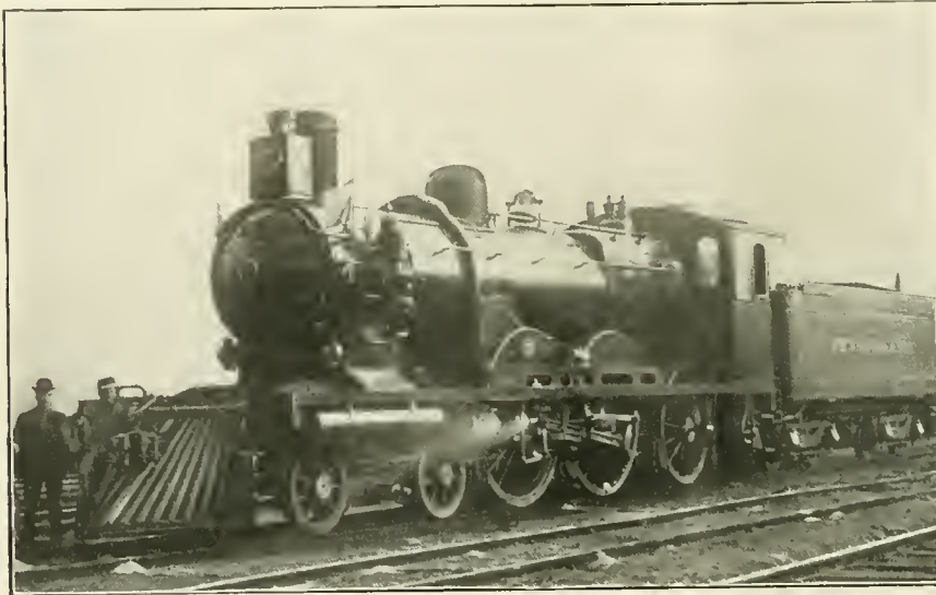
PENNSYLVANIA RAILROAD DE GLEHN COMPOUND.
